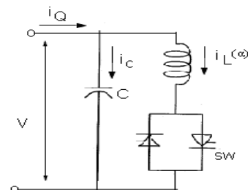
Fig.6. basic FC-TCR type static generator
