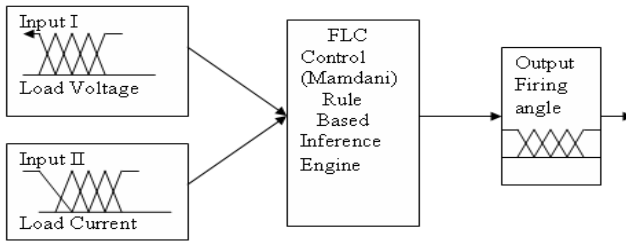
Fig.10. Structure of fuzzy logic controller
