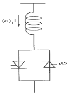
Fig. 1. Basic Thyristor Controlled Reactor
