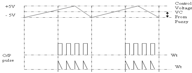
Fig.13.Generation of wave forms of TCA 785 IC
